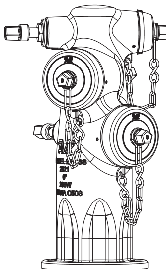
Series 243X-PPH 2 Pumper, 1 Hose Outlet
